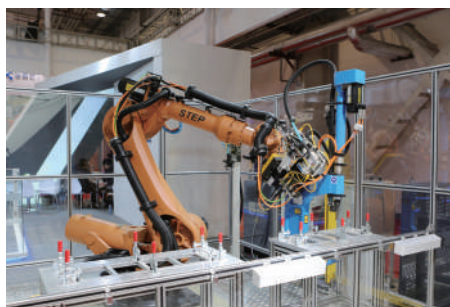
Riveting
