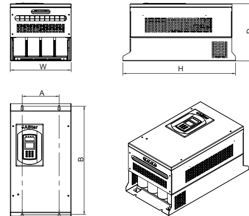
Inverter size diagram of A4-A9 specification
