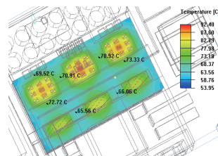
400kW air-cooled 680x350x110mm (length x width x height) Maximum temperature of radiator 82°C
