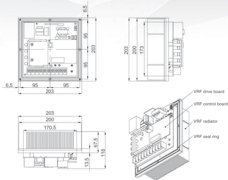
Drive board
