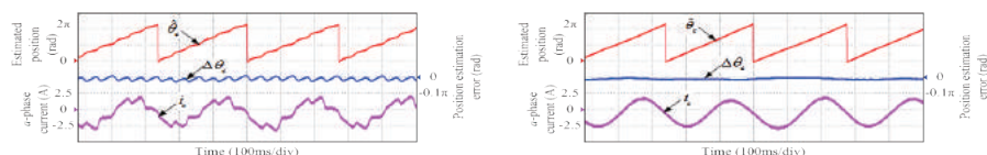
Angle error and phase current waveform before dead zone compensation
