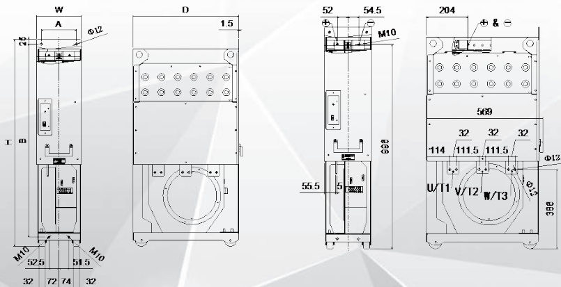
Main circuit terminal size of inverter drive unit
