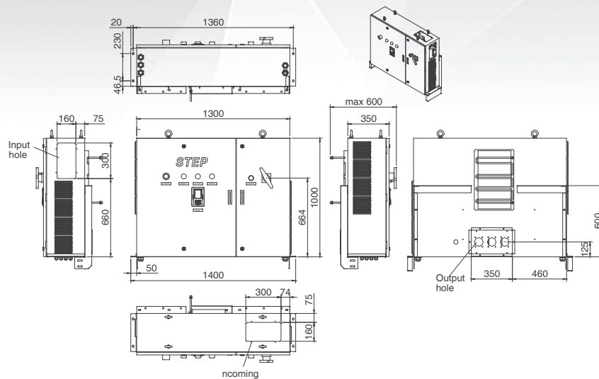
250kW-450kW boundary dimensions
