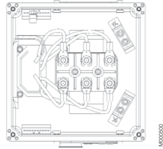
Terminal board for motor sizes 200 to 280
