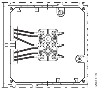
Terminal board for motor size 132
