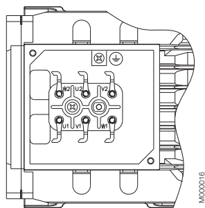
Terminal board for motor size 63
