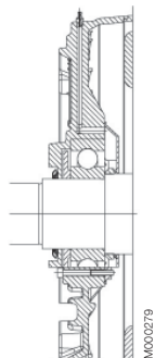
Motor sizes 160 - 250
