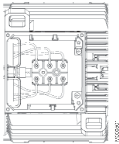
Terminal board for motor sizes 160 to 180
