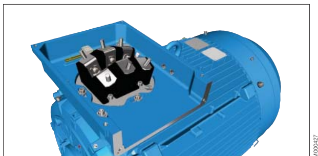
Fig. 8. Terminal board for motor sizes 280 - 315, except LKC.
