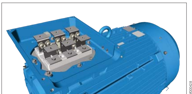
Fig. 10. Terminal board for motor sizes 315 LKC and 355 - 400.
