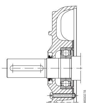
Motor sizes 71 - 132
