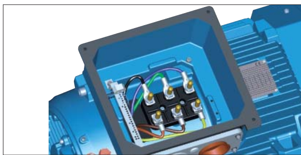
Fig. 6. Terminal board for motor sizes 160 - 250.
