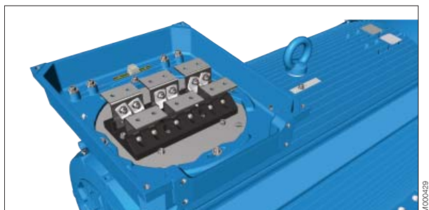
Fig. 12. Terminal board for motor size 450.
