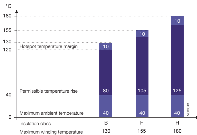
Safety margins per thermal class.
