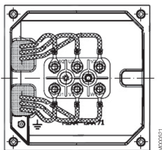
Terminal board for motor sizes 71 to 80
