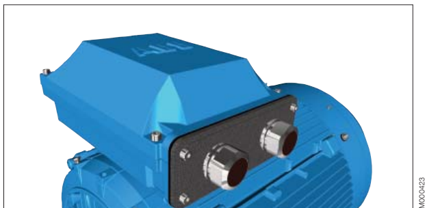
Fig. 7. Terminal box for motor sizes 280 - 315, except LKC. Connection flange with tapped cable entries.
